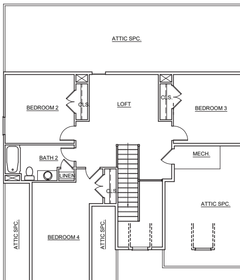
SECOND FLR. PLAN
