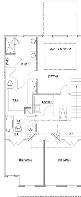
2nd Floor -Elevation C
