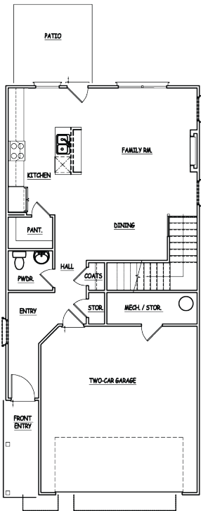
1st Floor
