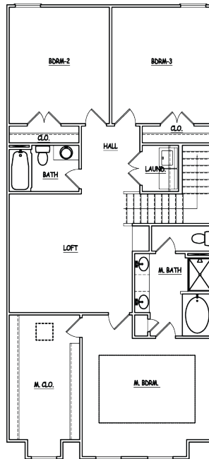
2nd Floor "A"
