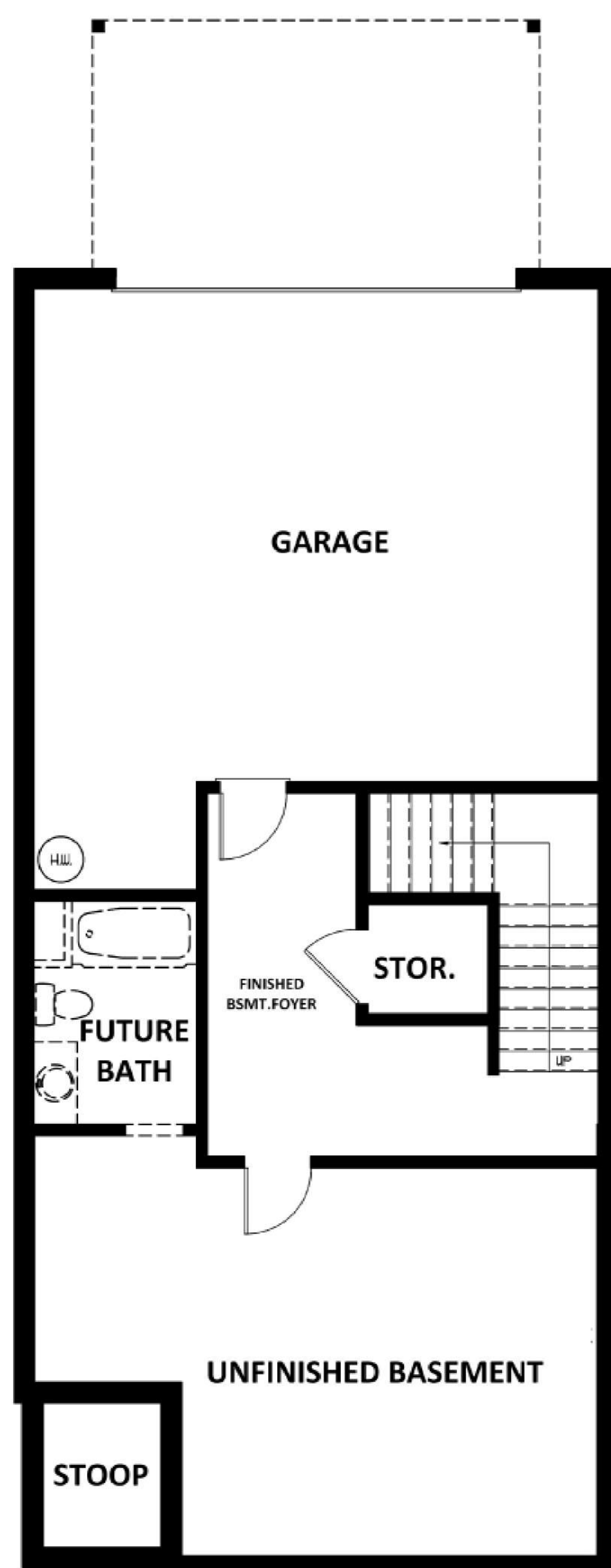
BASEMENT. FLOOR PLAN
