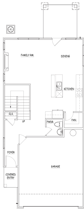
1st Floor
